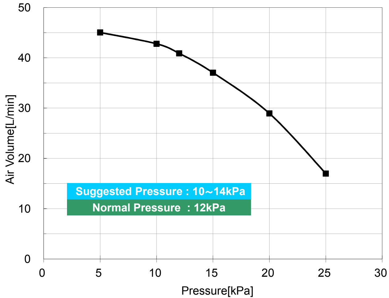
Performance Curve MAC40R (60Hz)
