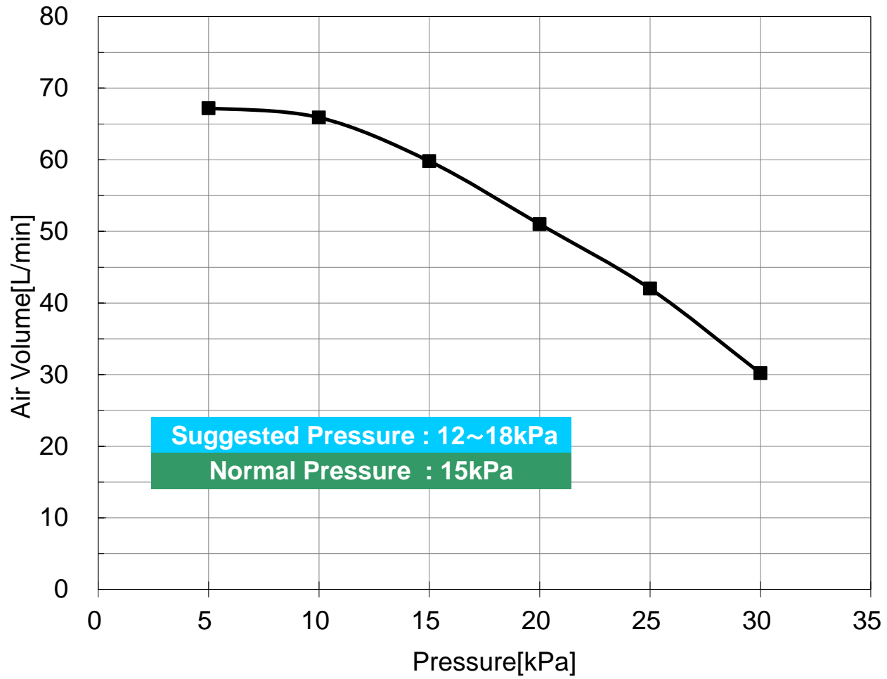
Performance Curve MAC60R (60Hz)
