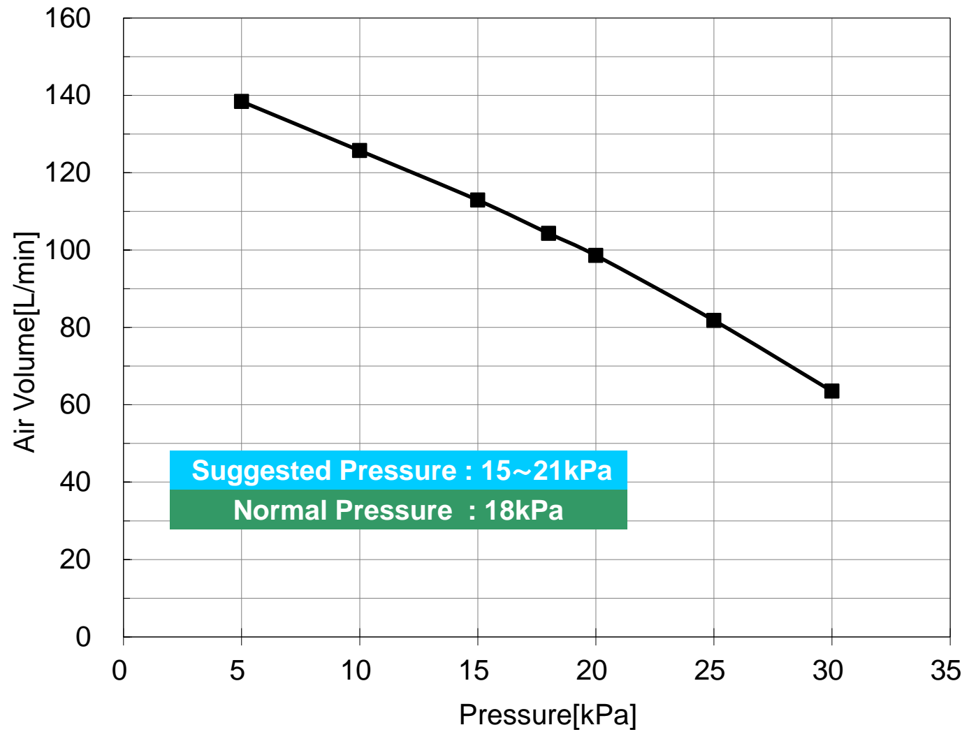
Performance Curve MAC100R (60Hz)
