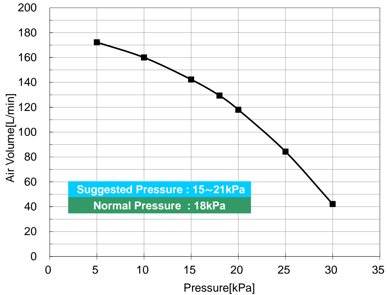
Performance Curve MAC120R (60Hz)
