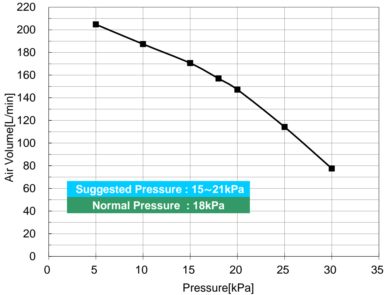
Performance Curve MAC150R (60Hz)
