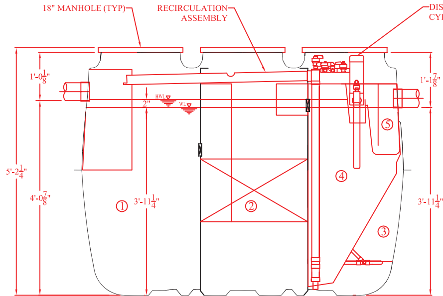
SECTION A-A VIEW
