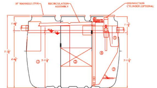
Structural drawings & tank details available for all models
