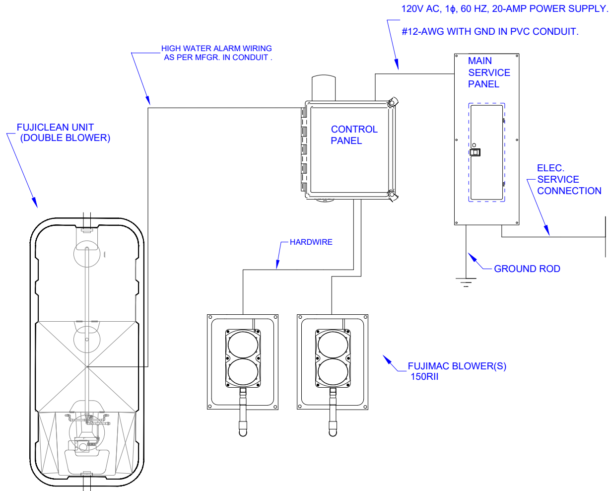
ELECTRICAL ONE LINE DIAGRAM SINGLE 2 BLOWER UNIT NOT TO SCALE
