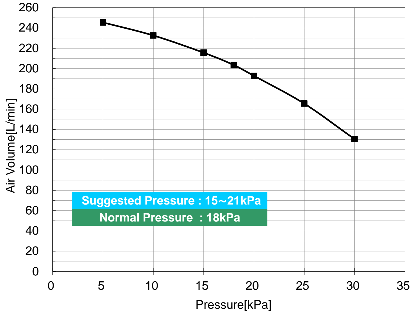
Performance Curve MAC200R (60Hz)
