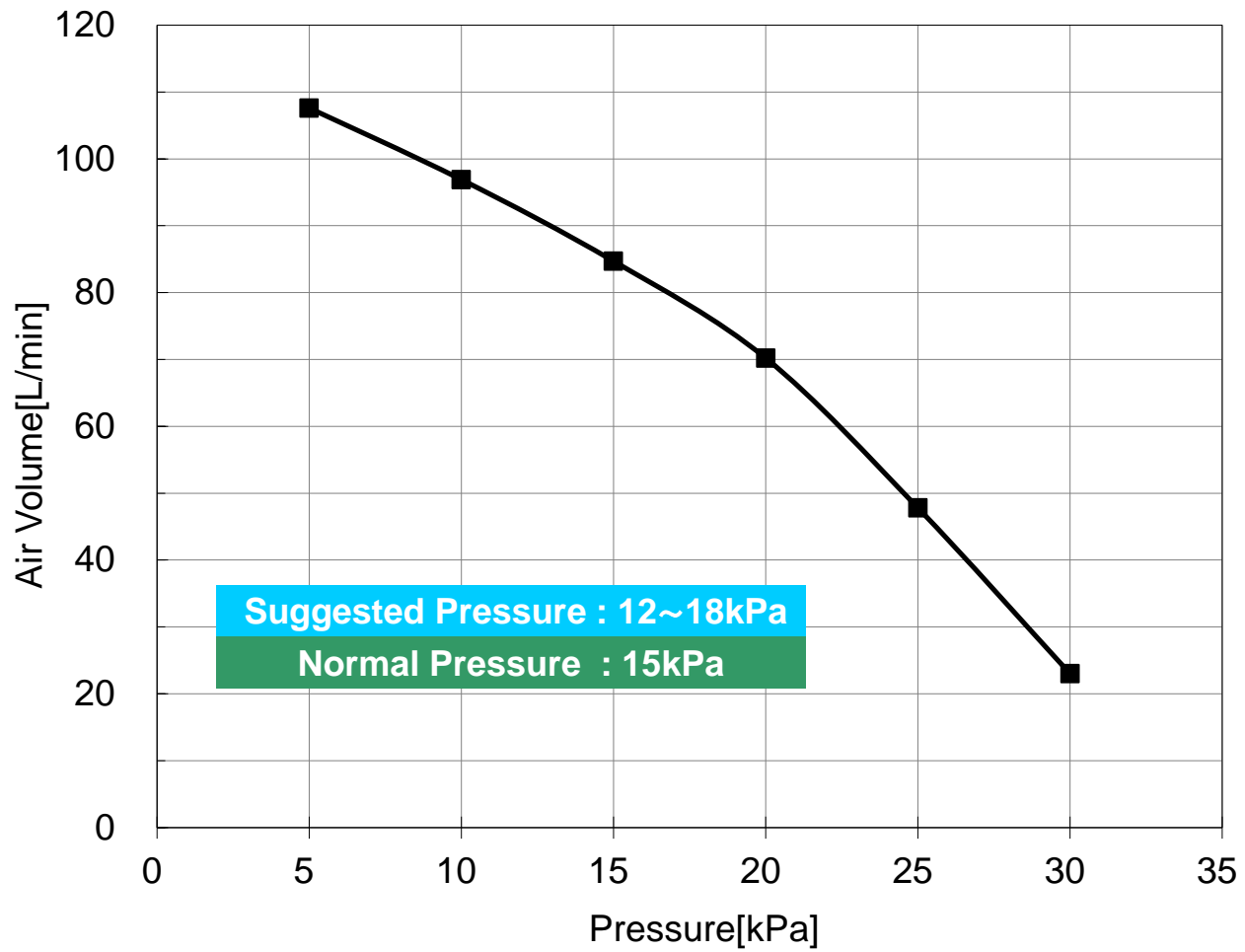
Performance Curve MAC80R (60Hz)
